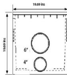
Catch Basin incl. galvanized dirt catcher
